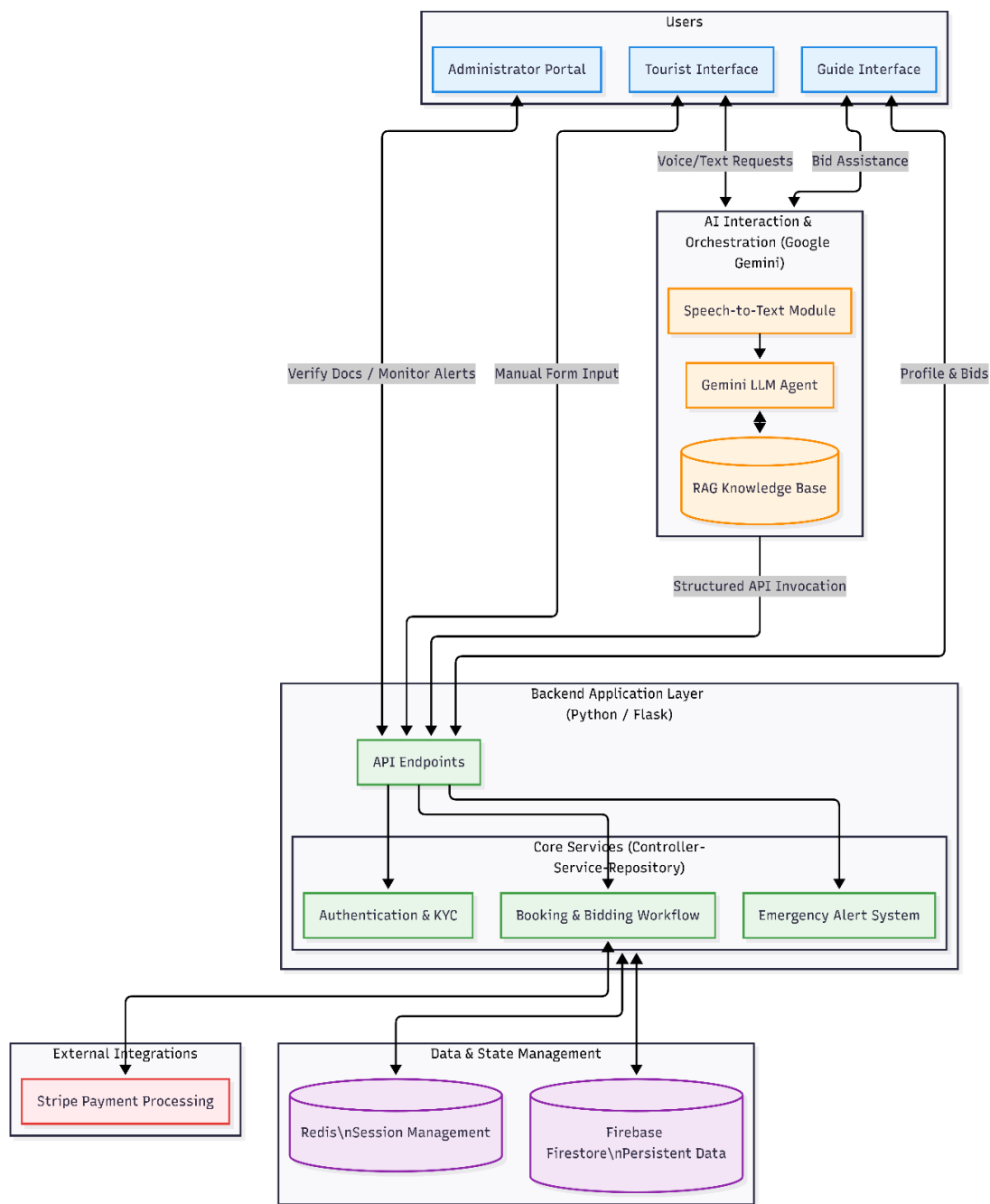
Figure 3 : Component Specific System Diagram
